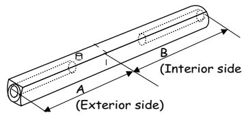
NXG-SCX Custom Straight Spindle
