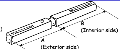
NXS-WCX Custom Swivel Spindle
